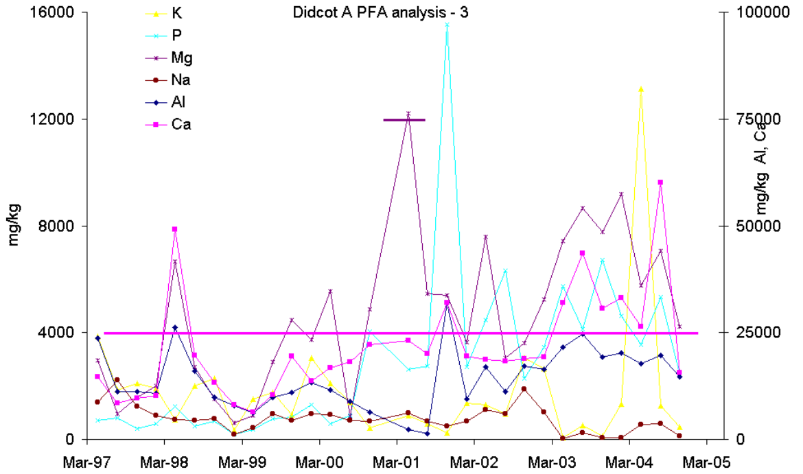
Figure A1.3 Analyses of PFA made at Didcot A Power Station (trigger levels indicated) Copyright © RWE npower 2005
